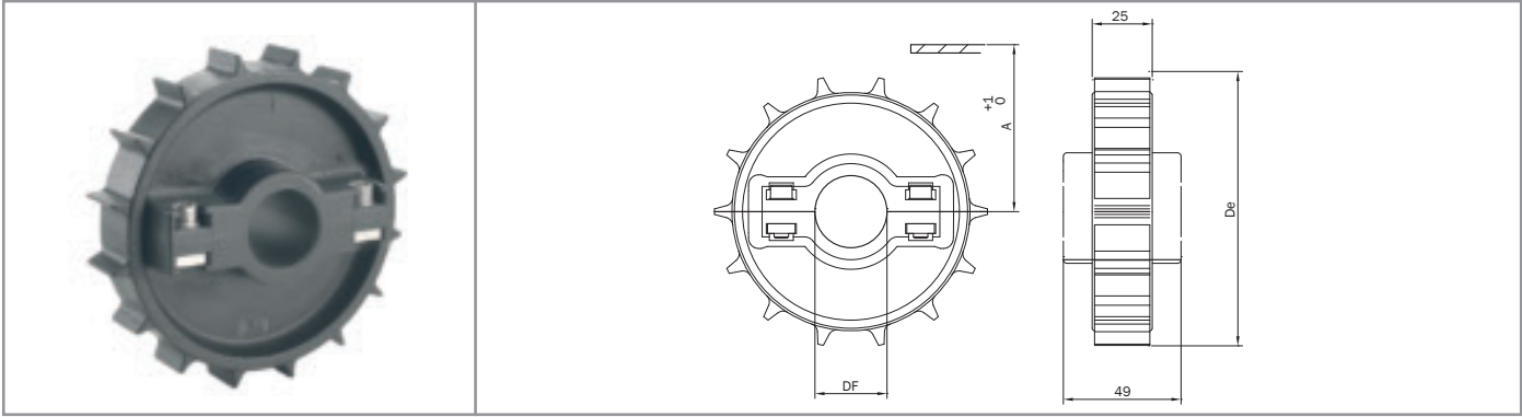
Split idler wheels material: reinforced polyamide - screw in stainless steel
