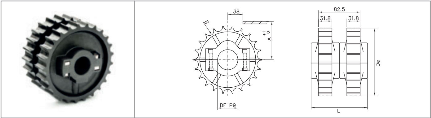
Split idler wheels material: reinforced polyamide - screws in stainless steel - nuts in nickel plated brass
