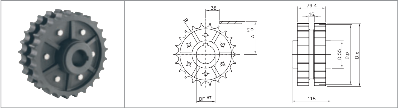
Drive sprockets material: reinforced polyamide - screws in stainless steel - UNI 6604 - 69 key seat
