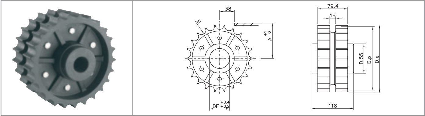
Standard idler wheels material: polyamide - screws in stainless steel - nuts in nickel plated brass
