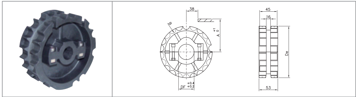
Split idler wheels material: polyamide - screws in stainless steel - nuts in nickel plated steel
