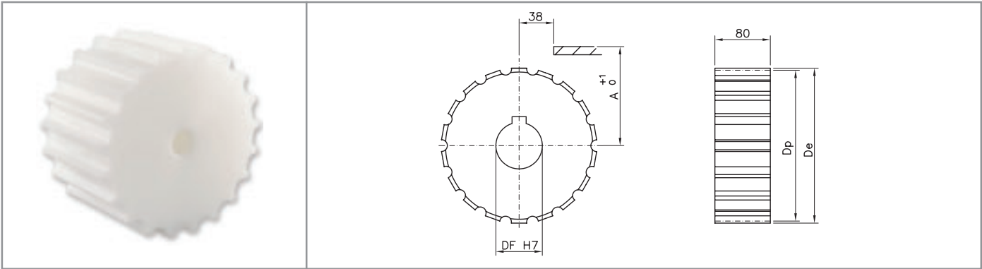
Standard sprockets material: polyamide - UNI 6604-69 key seat
