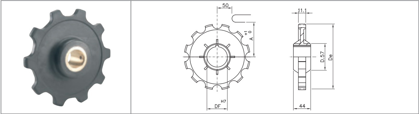
Standard sprockets material: polyamide, brass HUB - UNI 6604-69 key seat
