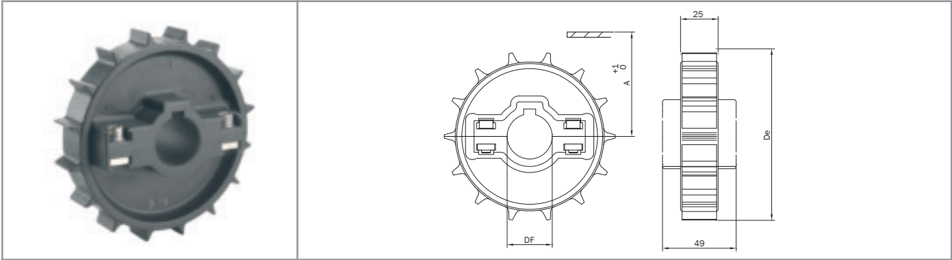
Split sprockets material: reinforced polyamide - screw in stainless steel UNI 6604-69 key seat
