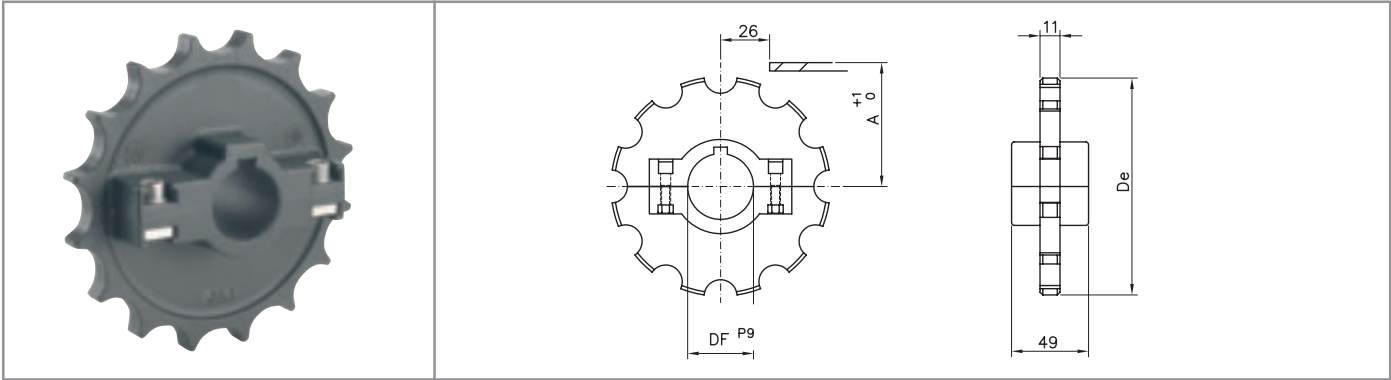
Split sprockets material: reinforced polyamide - screws in stainless steel - UNI 6604-69 key seat
