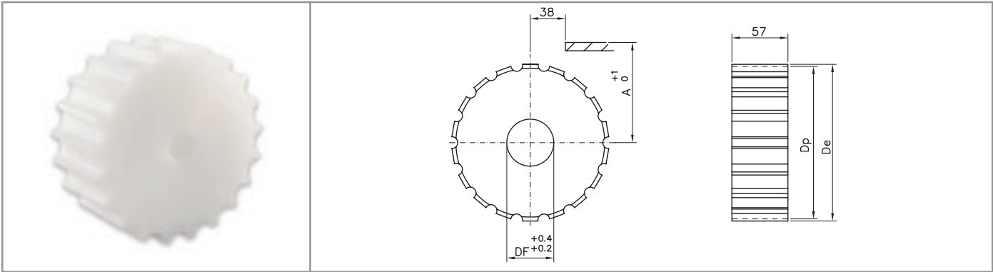
Standard idler wheels material: polyamide
